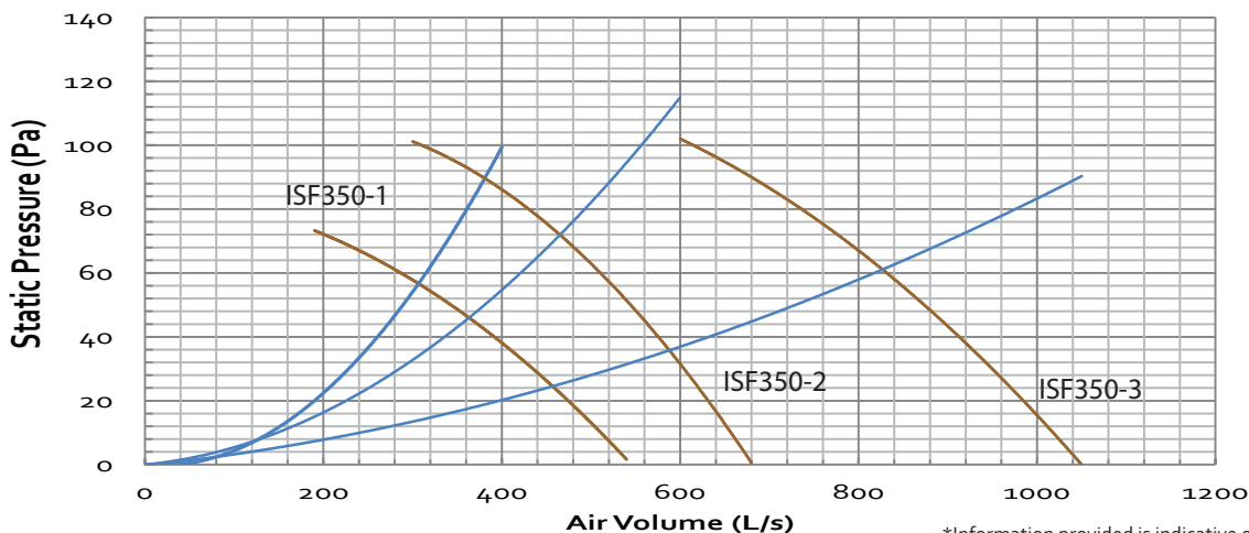
ISF350 Performance Curve
